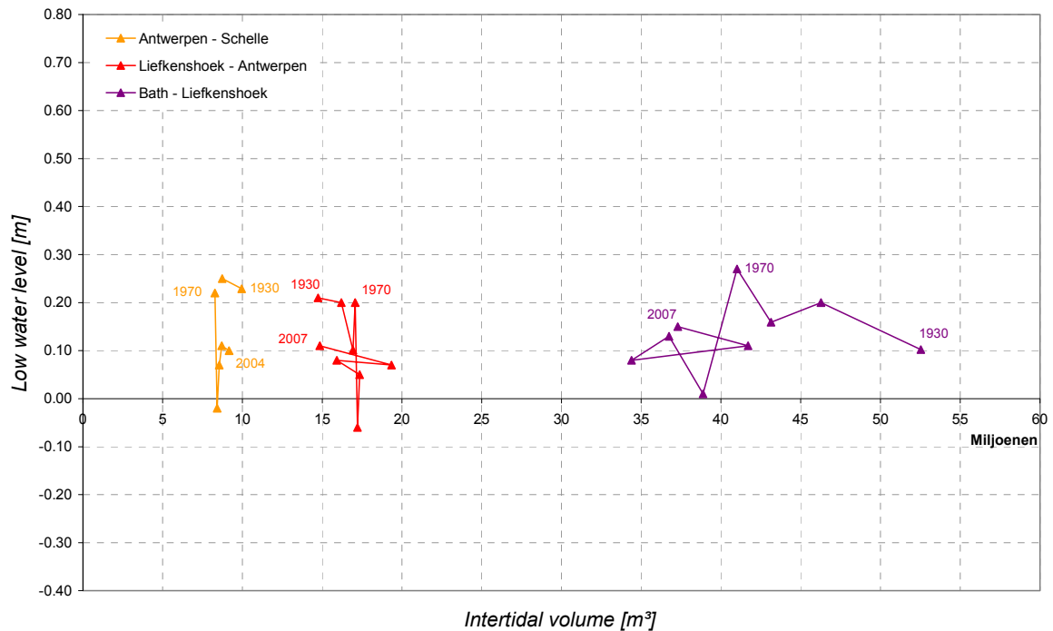
Figure 48 – Water volume of intertidal areas ( 0\text{m} < X < 6\text{m TAW} ) vs. low water level for different sections
