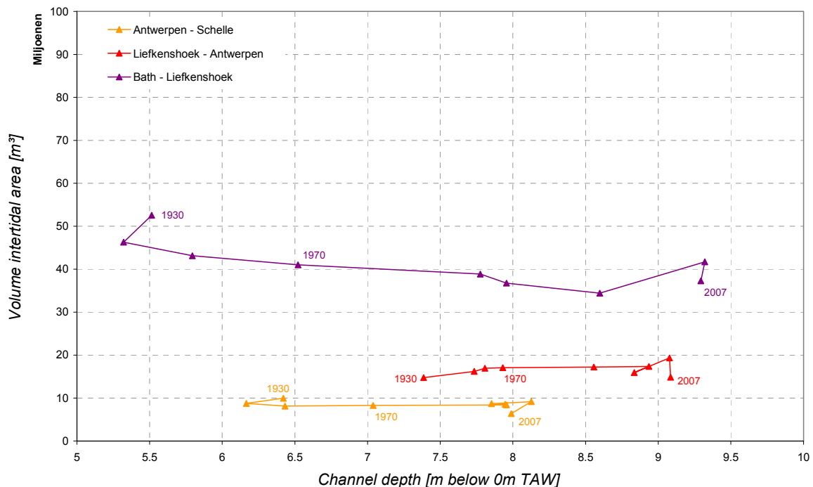
Figure 37 – Channel depth vs. water volume above intertidal areas ( 0\text{m} < X < 6\text{m TAW} ) for different sections
