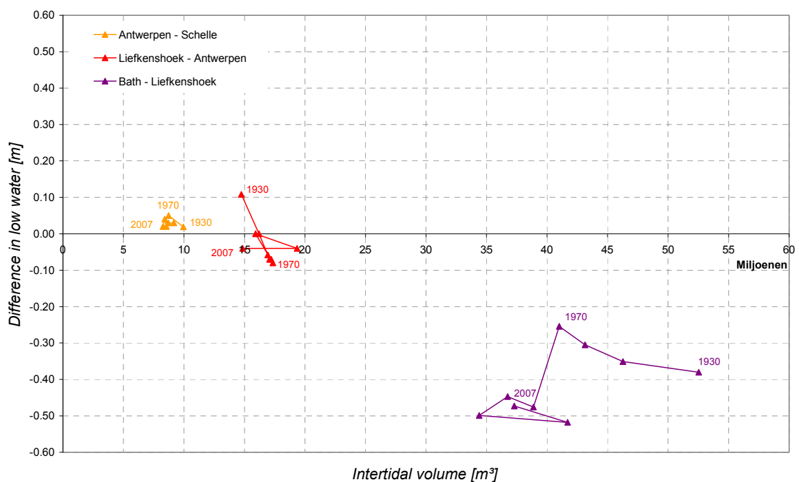
Figure 49 – Water volume of intertidal areas ( 0\text{m} < X < 6\text{m TAW} ) vs. difference of low water levels for different sections
