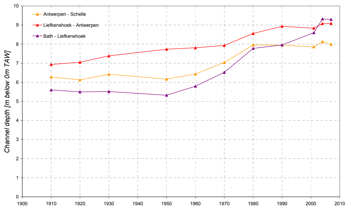
Figure 34 – Channel depth (&lt; 0m TAW) for different sections
