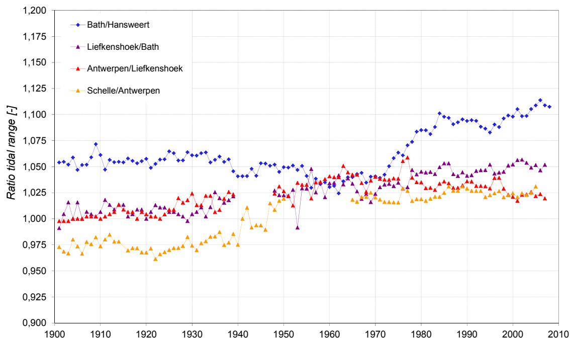
Figure 5 – Yearly-averaged ratio of tidal range in Bath, Liefkenshoek, Antwerpen and Schelle to tidal range in down-estuary station
