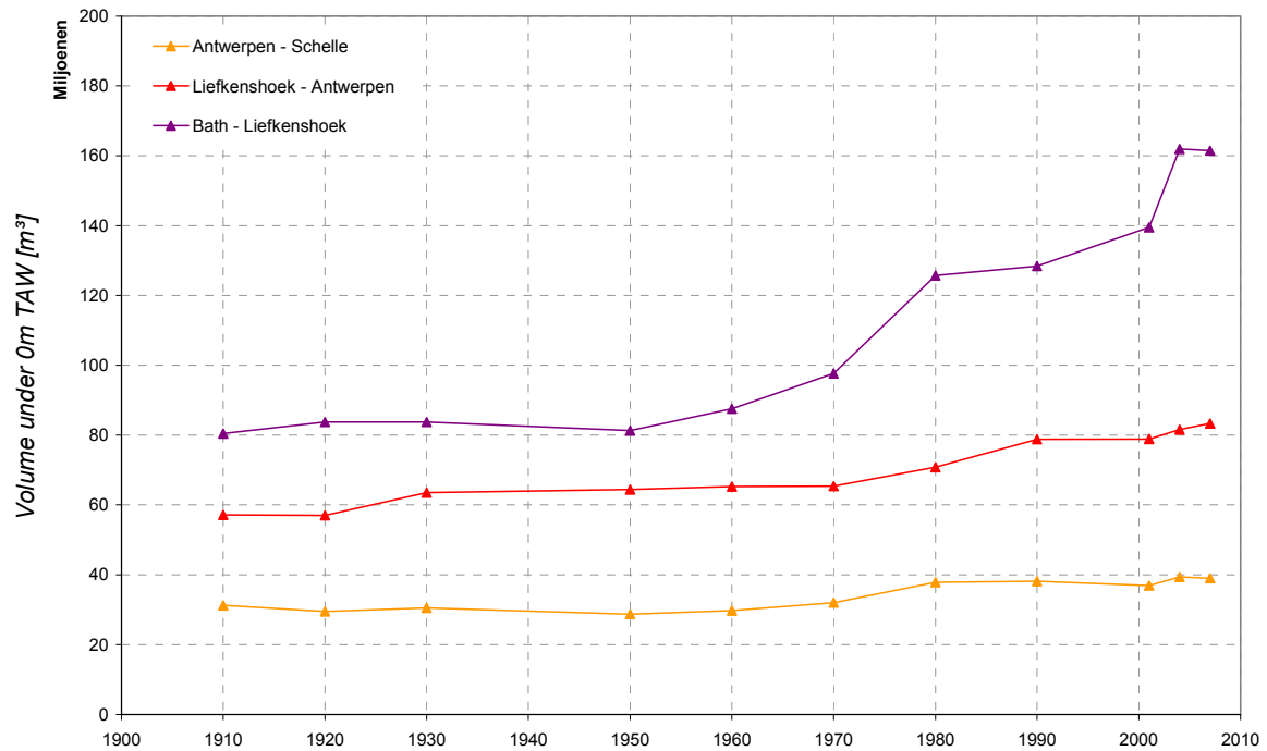
Figure 33 – Water volume of channel (&lt; 0m TAW) for different sections
