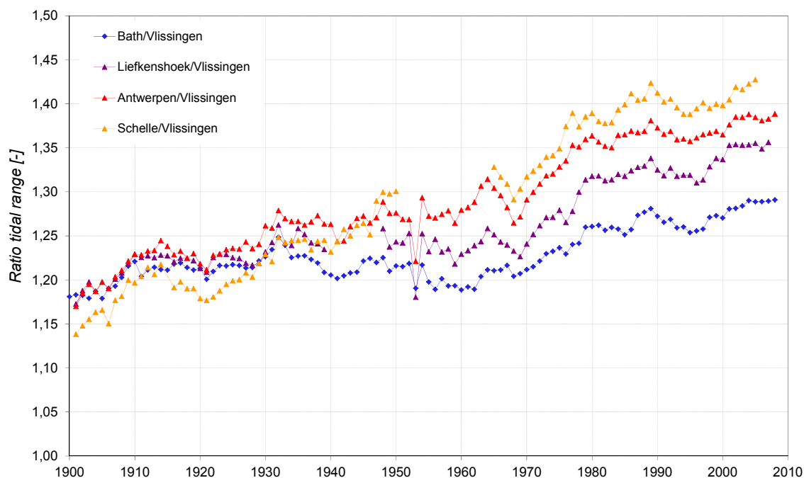
Figure 4 – Yearly-averaged ratio of tidal range in Bath, Liefkenshoek, Antwerpen and Schelle to tidal range in Vlissingen
